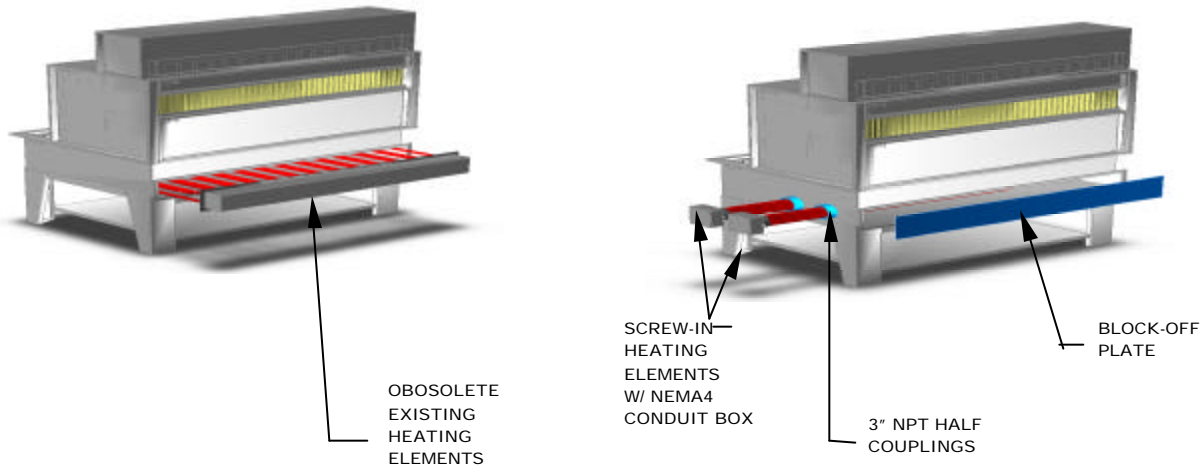
Older obsolete electric pan heaters
