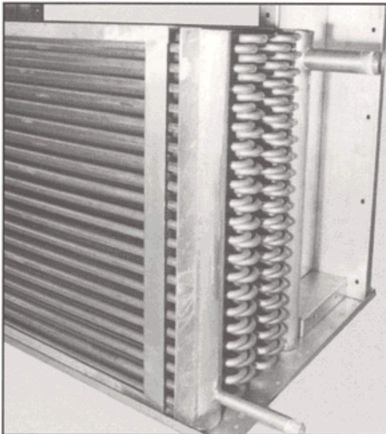
GEOMETRIC COIL ASSEMBLY
